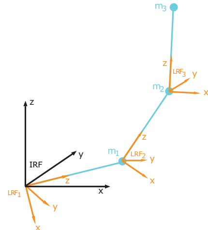
Fig. 3: Example of cable subdivision in three elements.
