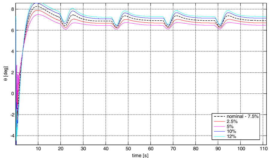
Fig. 13 The trend of the angle of pitch with different static margins (square pattern)
