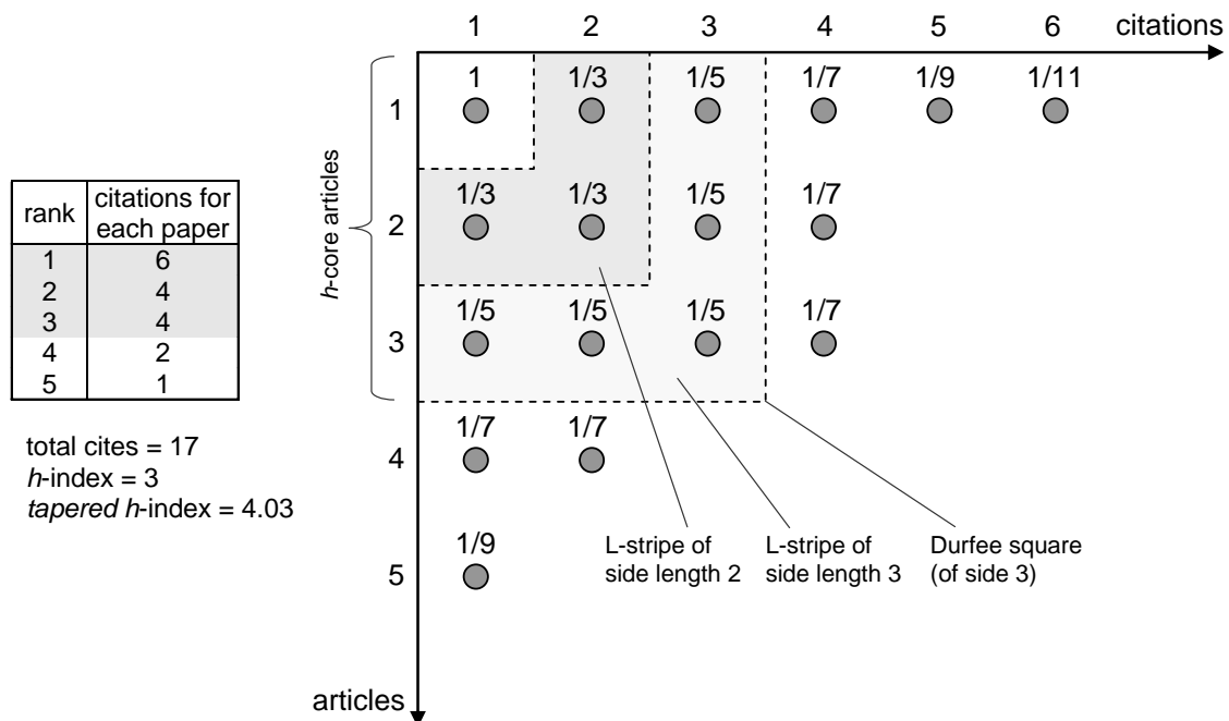
Fig. 1 – Example of a Ferrers diagram of an author’s citations. Adapted from Anderson et al. (2008).
