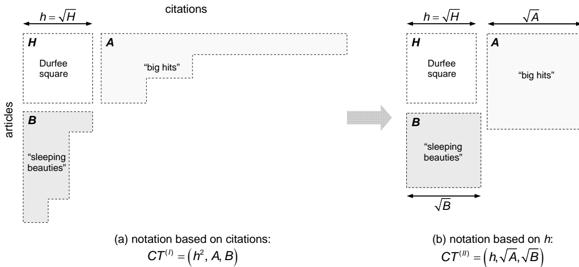
Fig. 8 – Graphical representation of the two possible notations for the citation triad. The first one – CT^{(I)} – is based on citations, whereas the second one – CT^{(II)} – is based on h .
