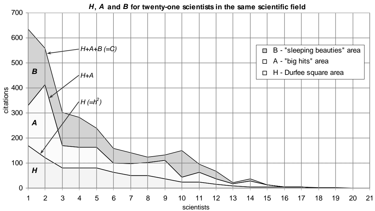
Fig. 9 – Chart representing the citation triad for the scientists in Tab. 1. Scientists are reported on the horizontal axis, while citation contributions ( H , A and B ) on the vertical axis. Conventionally, scientists are ranked in lexicographic order H \rightarrow C (sort according to H and, in case of equality, according to C=H+A+B ).
