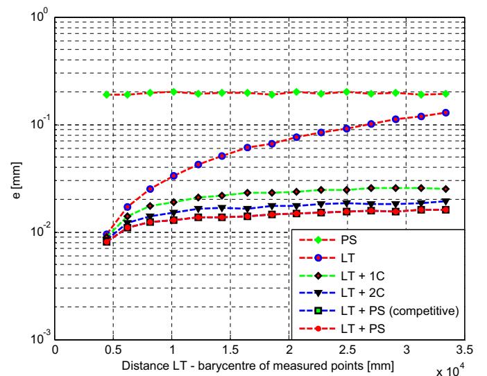
Fig. 2. Simulated mean absolute position error ( e ) versus the distance between the LT and the barycentre of measured points (LT: Laser tracker; PS: photogrammetric system; 1C: central camera of the photogrammetric system; 2C: two lateral cameras of the photogrammetric system).
