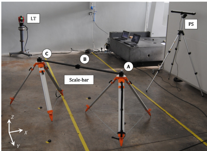
Fig. 1. Measurement layout (A, B and C are the reference points of the scale-bar).
