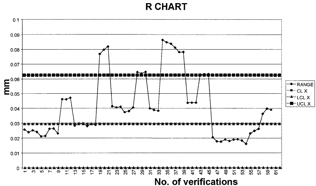
Figure 8. R chart of the reproducibility tests obtained by carrying out the positioning and measurement of several successive parts. The observed discontinuities reveal the effects of the introduced variability. For each measurement cycle three reproducibility tests have been carried out.
