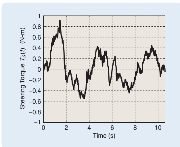
FIGURE 10 Controlled prototype. Steering torque T_\delta(t) applied to the handlebar axis of the controlled bicycle. The absolute value of the amplitude of the steering torque remains less than 1.5 N-m, corresponding to the maximum torque that can be provided by the servomotor.
