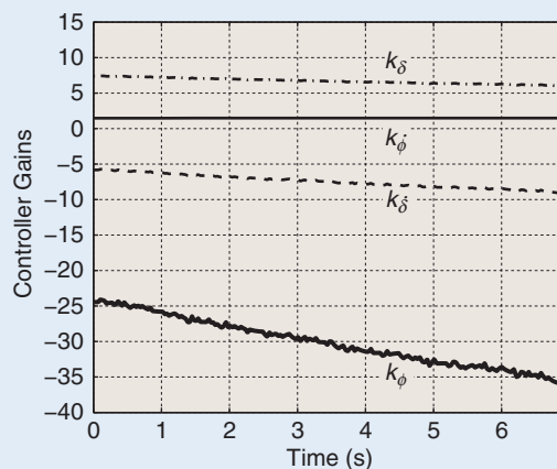
FIGURE 16 Controlled bicycle in the presence of an external impulsive roll-torque disturbance. Controller gains k_\phi [N-m/rad] (solid thick), k_\delta [N-m/rad] (dash-dot), k_{\dot{\delta}} [N-m-s/rad] (solid thin), k_{\ddot{\delta}} [N-m-s 2 /rad] (dashed). Although the gains k_\delta , k_{\dot{\delta}} , k_{\ddot{\delta}} are approximately constant, they are expected to vary with the bicycle speed, which is the scheduling variable of the linear-parameter-varying model describing the system dynamics. The controller gain k_\phi takes values between -25 [N-m/rad] and -35 [N-m/rad] when the bicycle speed ranges between 2.1 m/s and 1.6 m/s.
