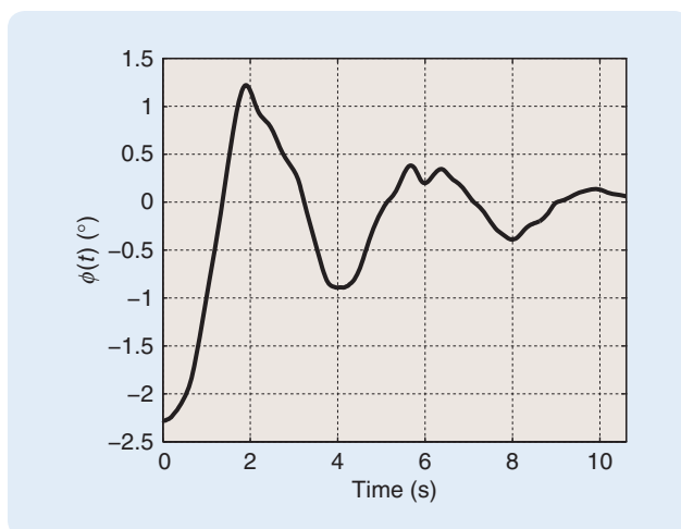
FIGURE 9 Controlled bicycle. Evolution of the roll angle \phi(t) . The prototype is pushed to the speed v(t) = 1.7 m/s. The test stops when the vehicle reaches the end of the room. After about 10 s, the amplitude of the bicycle roll angle is driven to 0.1^\circ starting from the initial condition -2.25^\circ . The designed linear-parameter-varying control system thus balances the riderless bicycle in the upright position.
