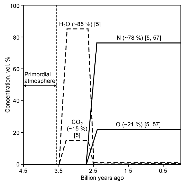
Fig. 5. Variations in the atmospheric composition over the Earth's life time. During the Archean era, about 15% of the Earth's atmosphere was constituted by \text{CO}_2 , and the remaining part was mainly composed of \text{H}_2\text{O} . The Earth's present atmospheric composition is dominated by nitrogen (N ~ 78%) and oxygen (O ~ 21%) [3, 57, 61, 62]
