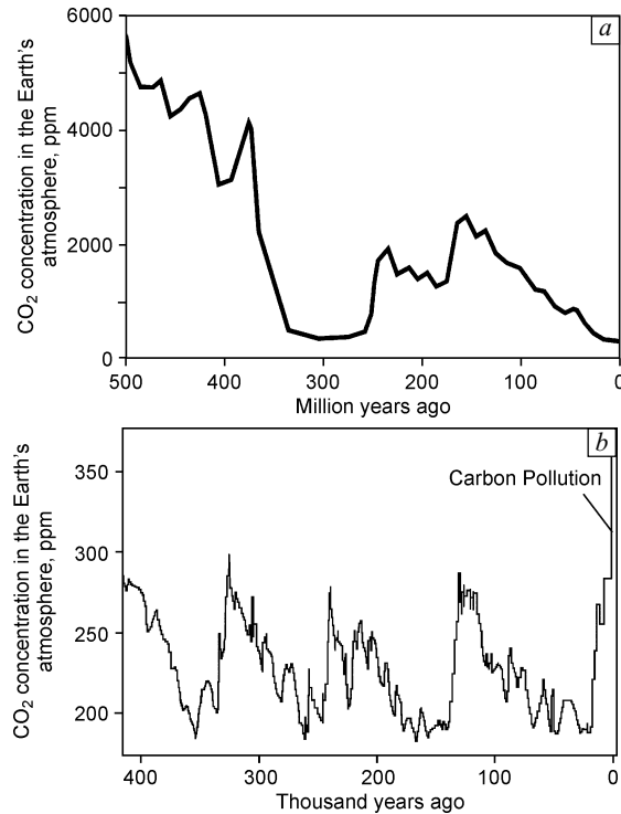
Fig. 6. a — CO 2 concentration in the Earth's atmosphere over the last 500 million years. The trend shown in the plot has been determined considering the database reported by Royer [63] together with the results of some geochemical models developed between 2001 and 2004 [64–68]; b — CO 2 concentration in the Earth's atmosphere over the last 4 \cdot 10^5 years [69, 70]
