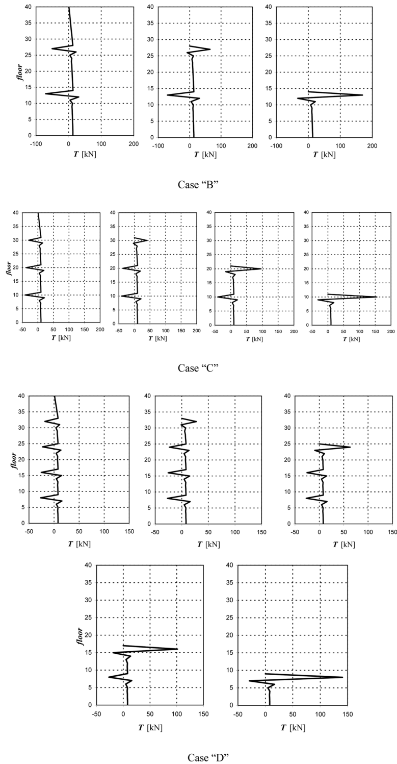
Fig. 18 Shear force distributions between bracings for the considered structures: "B", "C", and "D"
