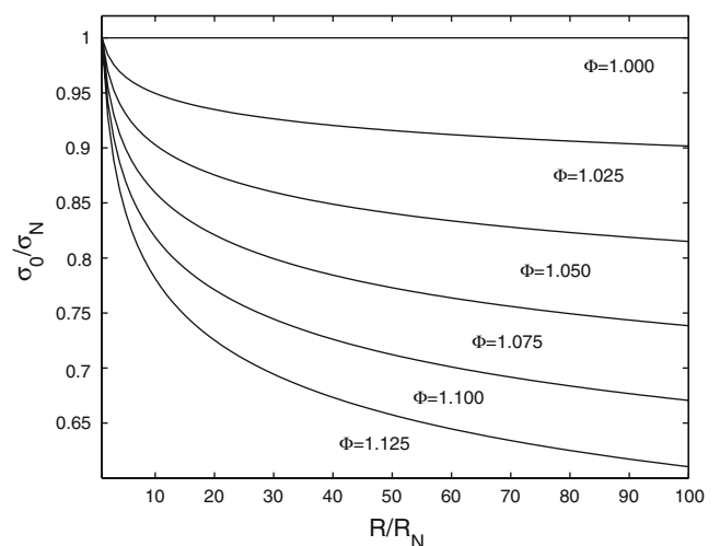
Fig. 3 Scaling law of the nominal strength \sigma_0 for different values of \Phi ( n = 9 , n_h = 8 )
