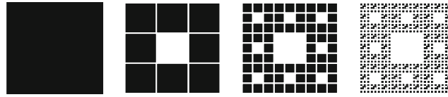
Fig. 2 The Sierpinski carpet ( D = 1.89 ) at different levels of observation; it corresponds to the cross section of a deterministic hierarchical bar in which the white zones represent the soft matrix and the black ones are the hard inclusions
