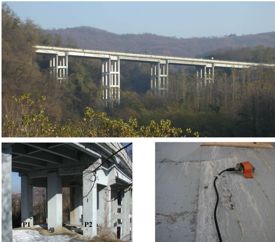
Fig. 10. The viaduct and the monitored pilasters P_1 and P_2 with the applied sensor.
