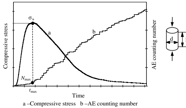
Fig. 13. Stress and cumulated event number versus time.
