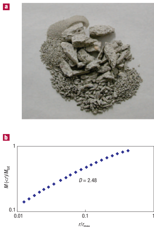
Figure 1 Fragment analysis. a , Often nature produces geometrical self-similar fragments, to maximize the entropy. These fragments were obtained by compression of a quasi-brittle material (concrete), and have a D value of around 2. b , Fragments of concrete obtained under artificial fragmentation (drilling), were analysed by computing the cumulative mass of particles with size smaller than r (divided by the total fragment mass) versus the same size r (divided by the size of the largest particle). Geometrical self-similar size distribution would appear as a straight line in this bilogarithmic diagram; from the slope, the fractal dimension can be deduced, here found to be close to 2.5.
