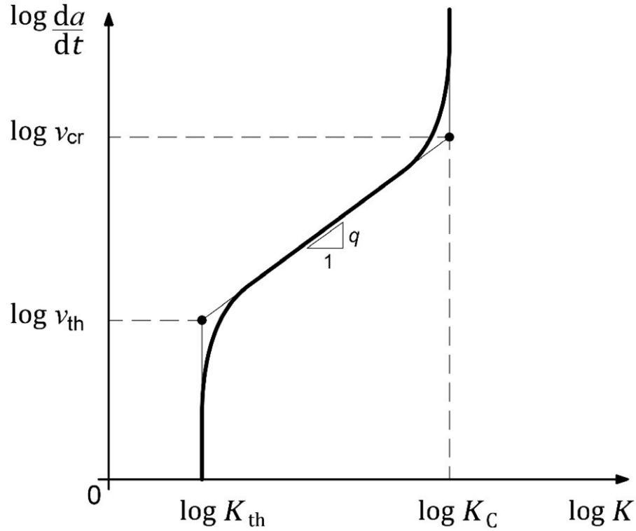
Fig. 3. Schematization of CCGR diagram: power-law stage corresponds to the intermediate asymptotic behaviour.
