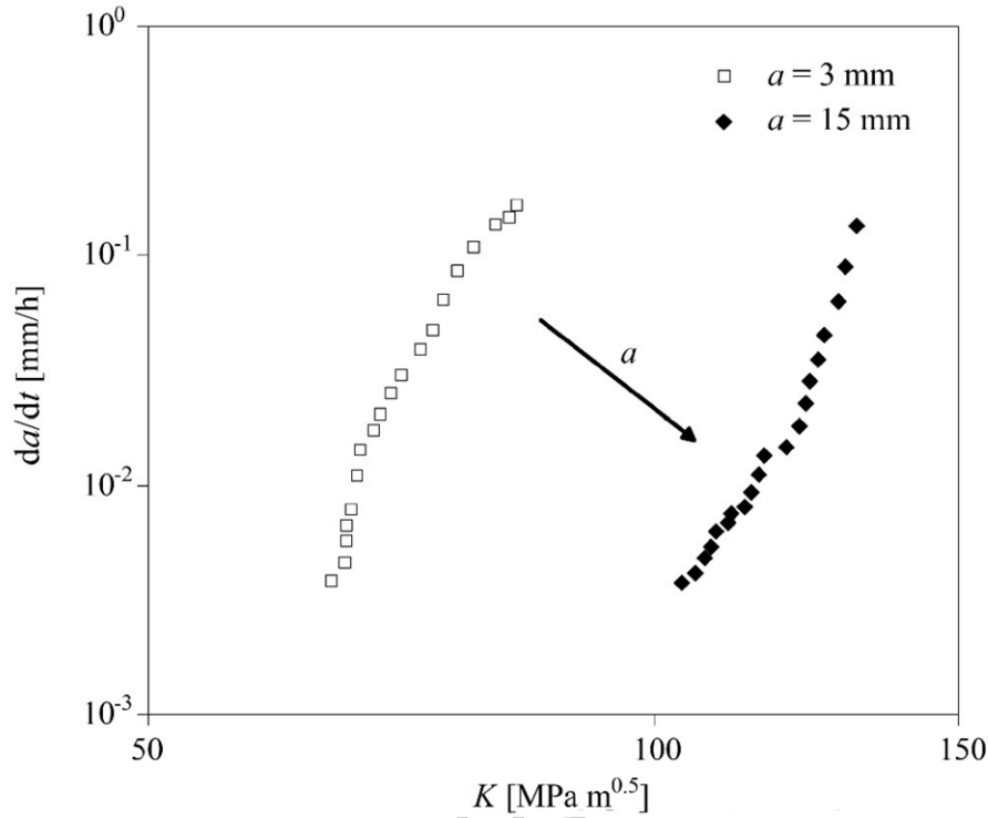
Fig. 2. Shift of experimental CCGR curves correlating da/dt with K (adapted from [41]) for different initial crack lengths, accounting for the crack-size effect.
