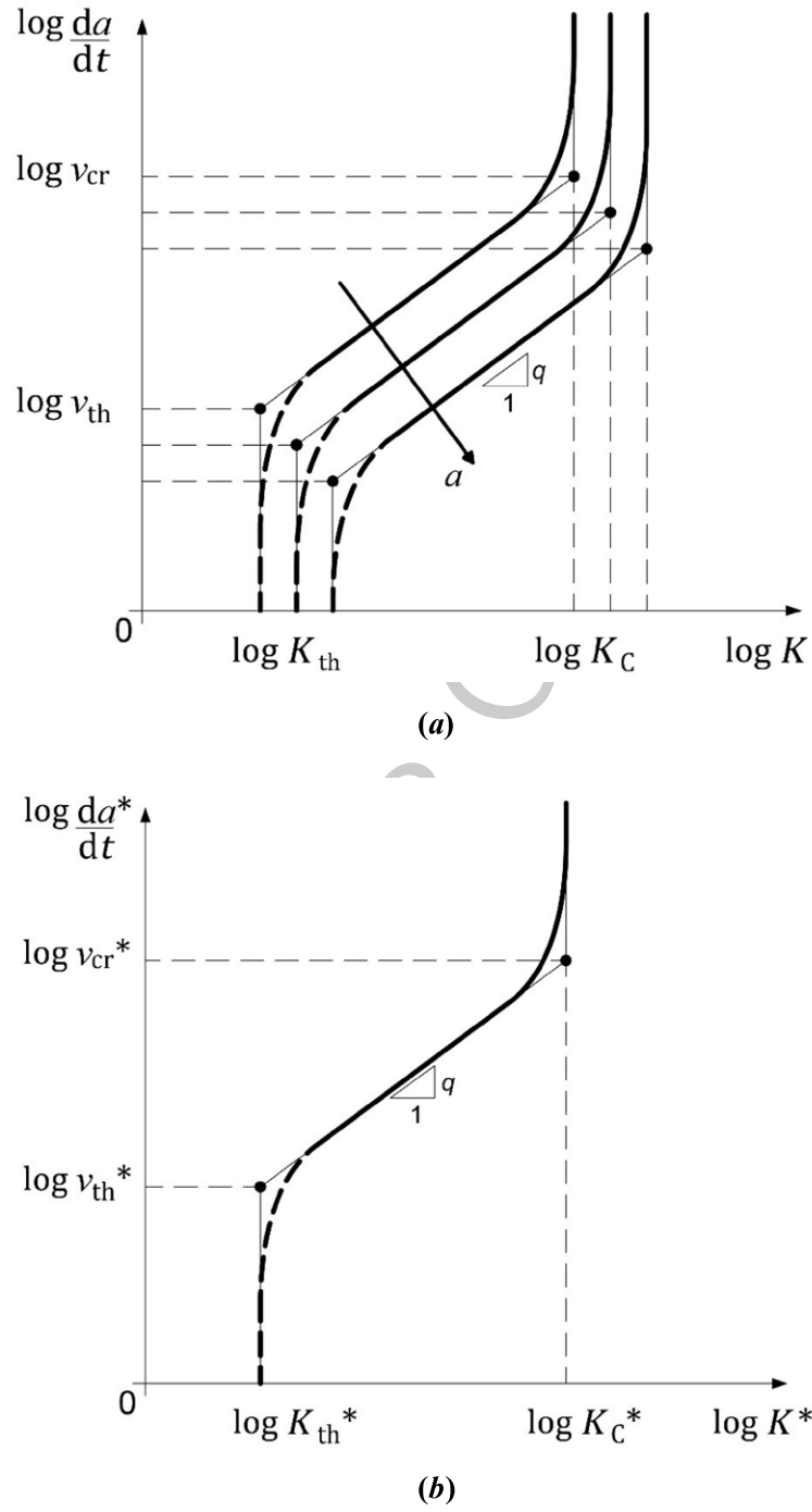
Fig. 5. Predicted nominal CCGR curves (a) and renormalized curve in the fractal diagram (b), where v_{th} (or v_{th}^* ) and v_{cr} (or v_{cr}^* ) denote threshold and critical CCGRs given by Eq. (14). The dashed line represents the region to be carefully investigated.
