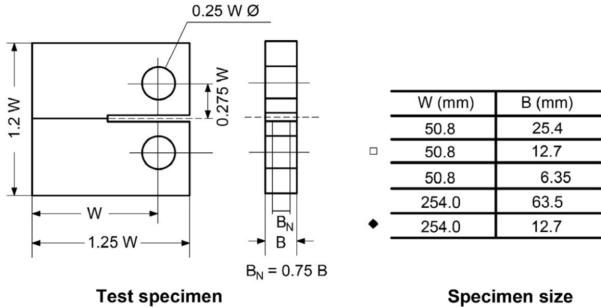
Fig. 1. Geometry and size of CT specimens tested (adapted from [41]).
