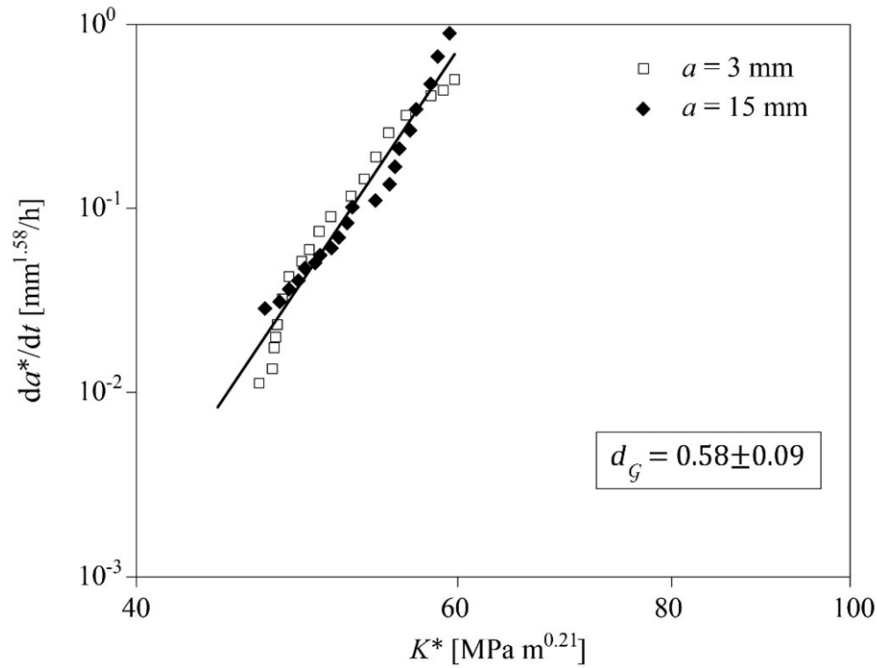
Fig. 4. Collapse of the renormalized CCGR data onto the fitting line represented by Eq. (18) in the fractal K^* vs da^*/dt diagram.
