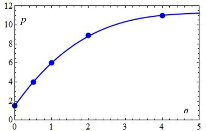
Fig. 10. Correspondence between the power law exponent n of the cohesive law and the parameter p defining the position of the (Dirac delta) weight function.
