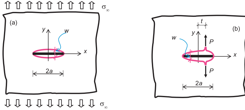
Fig. 1. Crack Opening Displacement for a crack of length 2a in an infinite slab subjected to: a remote uni-axial stress \sigma_\infty orthogonal to the crack (a); a pair of forces P acting on the crack faces (b).
