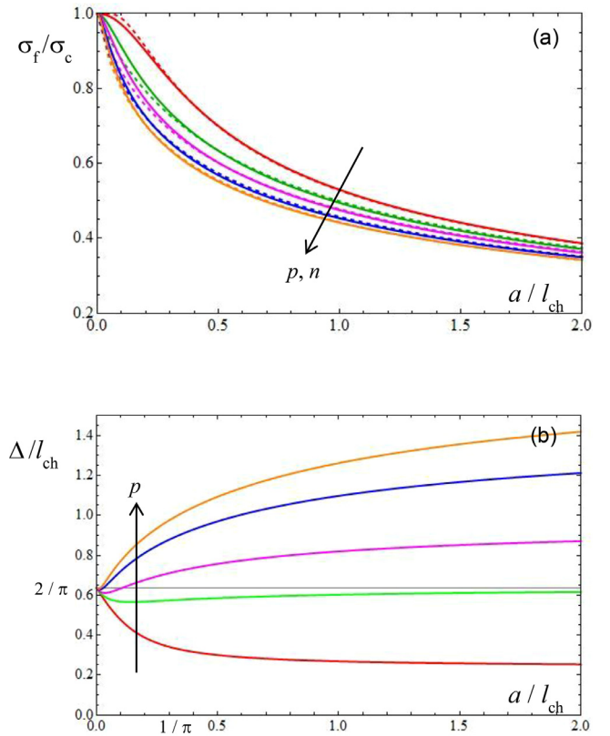
Fig. 9. Failure stress vs. crack length (a) according to FFM – continuous lines – and to CCM – dotted lines; finite crack advancement vs. crack length (b). FFM and CCM plots correspond respectively to the following values: p=1.5, 4, 6, 9, 11 and n=0, 0.5, 1, 2, 4 .
