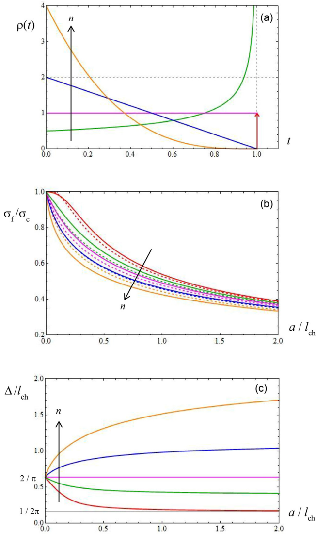
Fig. 8. Stress weight functions (a); failure stress vs. crack length according to FFM (continuous lines) and CCM (dotted lines) (b); finite crack advancement vs. crack length (c). Curves correspond to the following values: n=0, 0.5, 1, 2, 4 .
