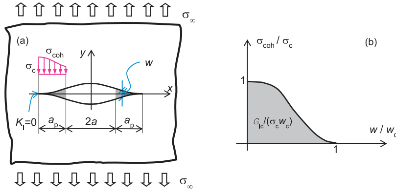
Fig. 2. Cohesive crack model for a crack of length 2a in an infinite slab subjected to a remote uni-axial stress \sigma_\infty : details of the process zone and of the cohesive stresses (a); generic cohesive law (b).
