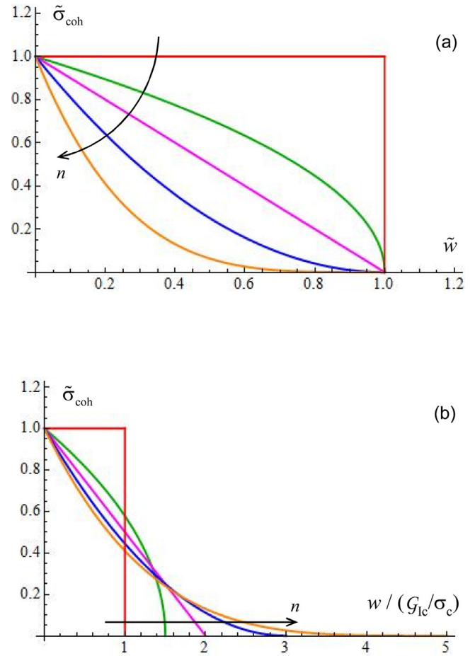
Fig. 4. Cohesive laws with power law softening for: constant tensile strength and constant critical displacement (a); constant tensile strength and constant fracture energy (b). Cohesive laws are plotted for the following power law exponent values: n = 0, 0.5, 1, 2, 4 .
