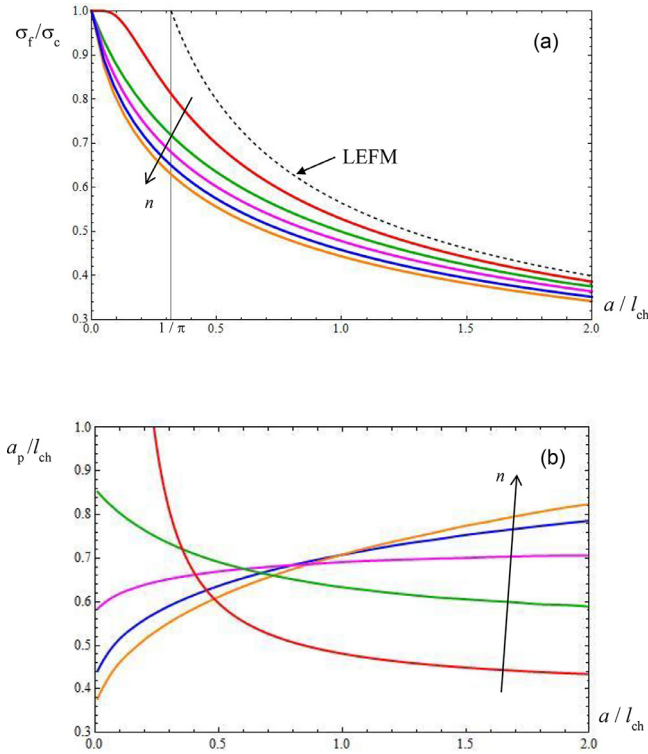
Fig. 5. Failure stress vs. crack length (a) and process zone size (at \sigma_\infty = \sigma_f ) vs. crack length (b) for cohesive laws with different power law exponent ( n=0, 0.5, 1, 2, 4 ).
