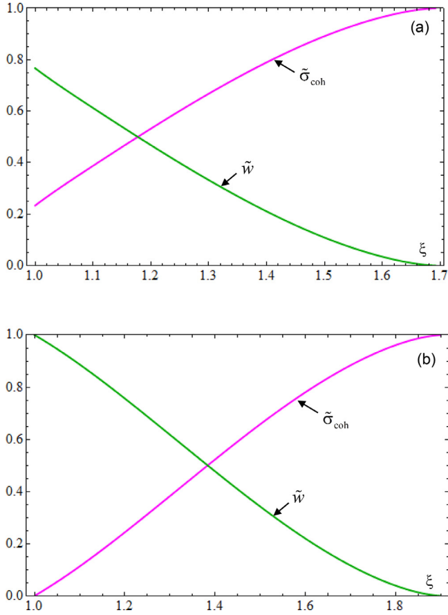
Fig. 3. Normalized cohesive stresses and opening displacement within the process zone for \alpha = 1 and linear softening; real crack tip on the left ( \xi = 1 ) and fictitious crack tip on the right ( \xi = \beta ): (a) \beta = 1.691 , corresponding to the maximum remote stress ( \sigma_f = 0.478 \sigma_c ); (b) \beta = 1.899 , corresponding to real crack growth onset.
