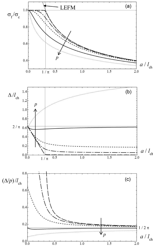
Fig. 7. Failure stress vs. crack length (a) according to FFM with different p values ( p = 0.01, 0.3, 1, 4, 12 ); finite crack advancement vs. crack length (b); length where stress exceeds \sigma_c vs. crack length (c). Curves with the same dashed refer to the same p value.
