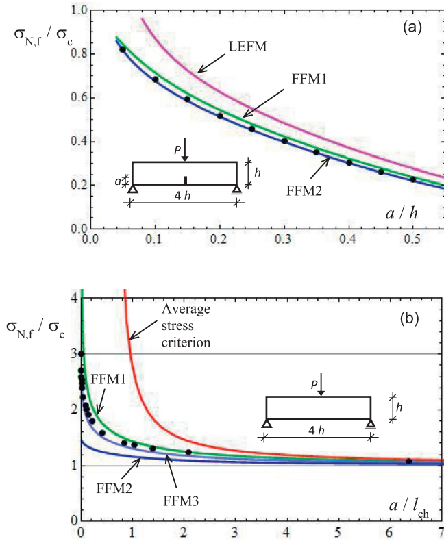
Fig. 11. Dimensionless nominal stress at failure vs. relative crack depth for TPB cracked beams for h/l_{ch} = 4.14 (a): LEFM (magenta line); FFM1, with uniform weight function (green line); FFM2, with Dirac weight function having p=6 (blue line); CCM, with linear softening (black dots – from Carpinteri and Colombo, 1989 ). Nominal stress at failure vs. size, dimensionless plot (b): average stress criterion (red line); FFM1, with uniform weight function (green line); FFM2, with Dirac weight function having p=6 (blue line); FFM3, with Dirac weight function having p=3 (light blue line); CCM, with linear softening (black dots – from Carpinteri and Colombo, 1989 ). (For interpretation of the references to color in this figure legend, the reader is referred to the web version of this article.)
