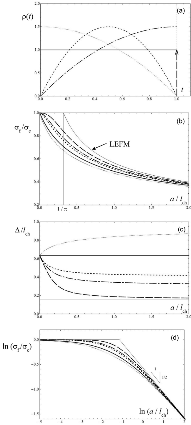
Fig. 6. Stress weight functions (a); failure stress vs. crack length (b); finite crack advancement vs. crack length (c); failure stress vs. crack length, bi-logarithmic plot (d). Plots in (b,c,d) refer to weight functions in (a) having the same dashed: \rho(t) = -1.5(1-t^2) , dotted line; \rho(t)=1 , continuous line; \rho(t)=6t(1-t) , short-dashed line; \rho(t)=-1.5t(2-t) , dot-dashed line; \rho(t)=\delta(1-t) , long-dashed line.
