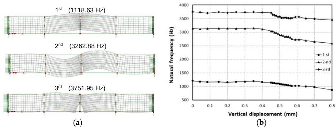
Figure 9. Test 1: (a) first three numerical (FEM) bending modes and related frequencies (unloaded beam, initial notch depth) and (b) experimental natural frequencies vs. displacement curves.
