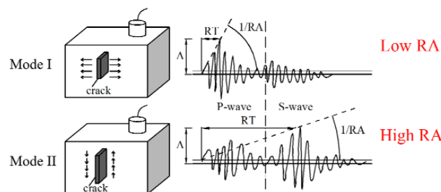
Figure 1. Typical waveforms for tensile and shear events. A is the amplitude and RT is the rise time (time between the onset and the point of maximum amplitude) of the waveforms. Reproduced with permission from [7], Elsevier, 2016.
