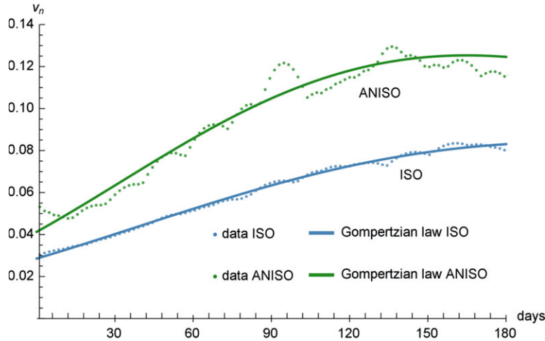
FIGURE 5 Maximum value of expansion velocity v_n of the tumour front over time, monitored in the isotropic homogeneous (ISO) and anisotropic heterogeneous (ANISO) simulations. The dots correspond to the numerical values of the front velocity recorded along the direction orthogonal to the tumour front, i.e. v_n := \max_{\mathbf{x}_j} \mathbf{V} \cdot \mathbf{n} , where \mathbf{V} is defined in (23) and \mathbf{n} is the direction orthogonal to the tumour front. The solid lines are the fitting of the numerical data with a Gompertz curve v_n = rck \exp(-c \exp(-rt)) \exp(-rt) , with k = 15.3944 \pm 0.0916 , c = 3.2626 \pm 0.0034 , r = 0.0056 \pm 2.52 \text{ e-}5 in the IS case, and k = 47.9809 \pm 0.3333 , c = 3.3060 \pm 0.0116 , r = 0.0071 \pm 4.76 \text{ e-}5 in the AN case, calculated by a non-linear least-squares fitting method
